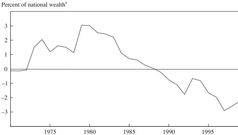
Figure 3. Share of U.S. Net Foreign Assets in the Country Portfolio, 1970–99
