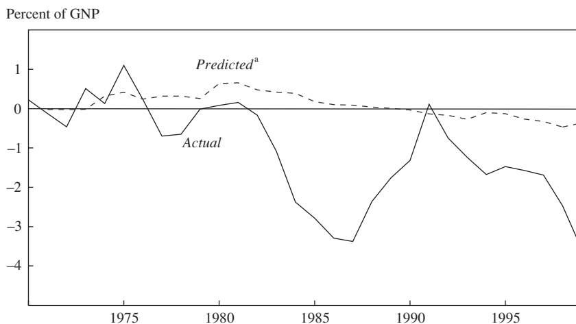
Figure 1. Actual and Predicted U.S. Current Account Balance, 1970–99
